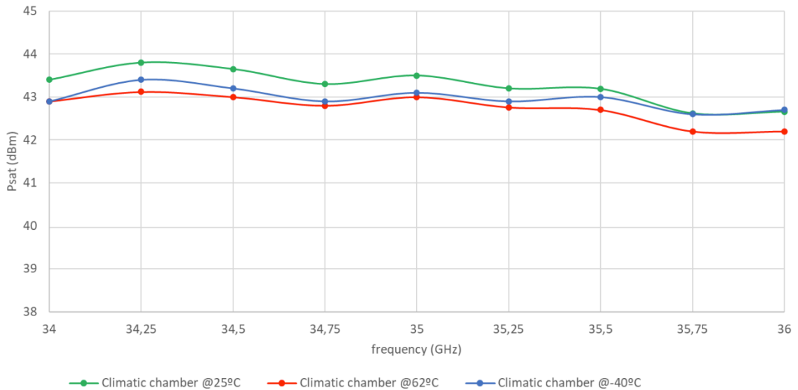
Figure 1: ERZ-HPA-3400-3600-43 P_{sat}
