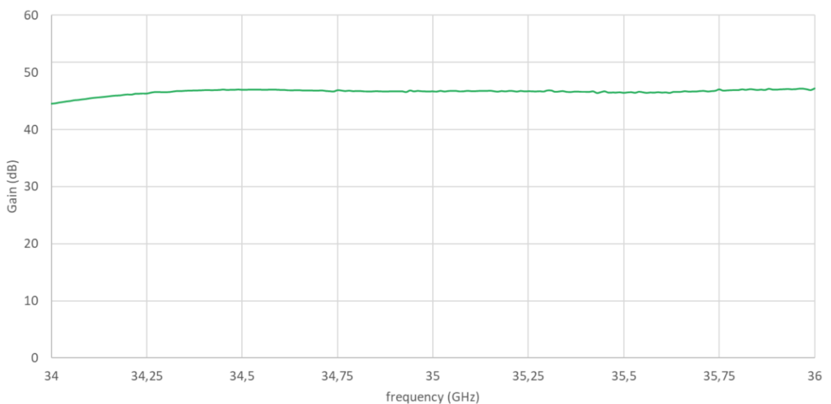
Figure 2: ERZ-HPA-3400-3600-43 Small Signal Gain
