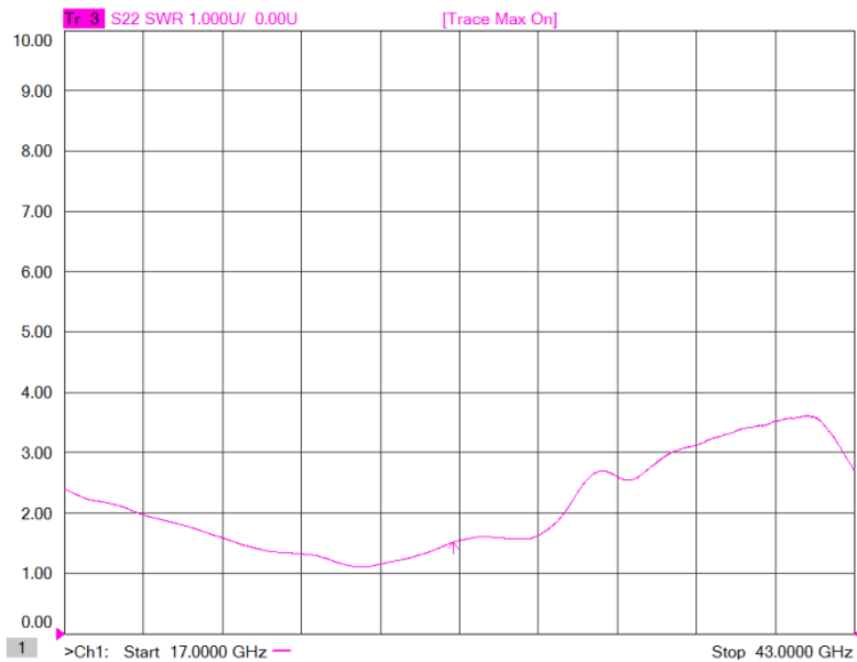
Figure 4: ERZ-HPA-1700-4300-22 Output Matching
