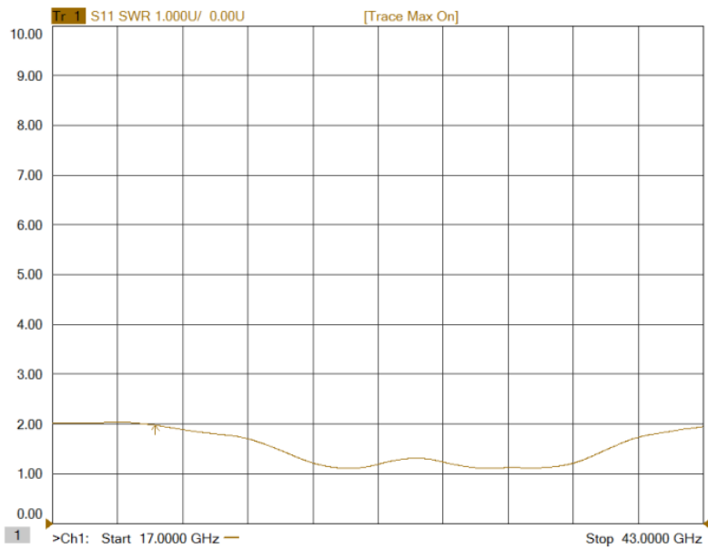
Figure 3: ERZ-HPA-1700-4300-22 Input Matching
