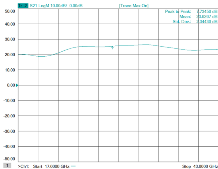
Figure 2: ERZ-HPA-1700-4300-22 Small Signal Gain
