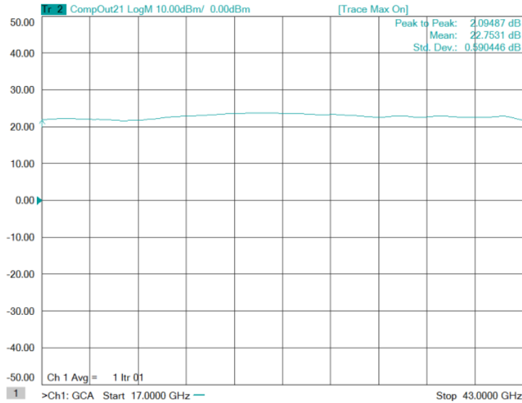
Figure 1: ERZ-HPA-1700-4300-22 Psat
