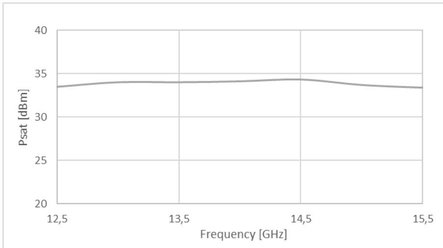
Figure 1: ERZ-HPA-1250-1550-34 Psat
