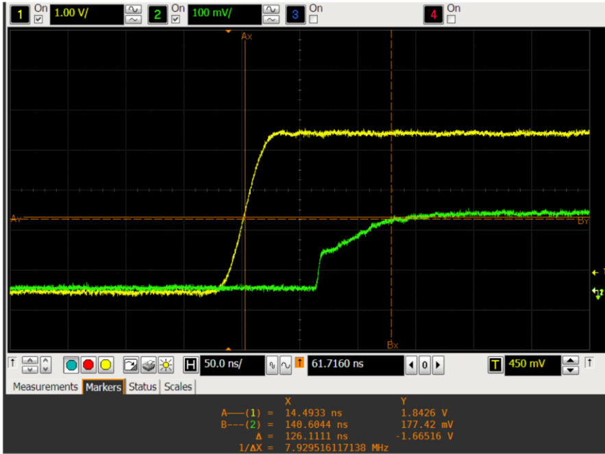
Figure 7: ERZ-HPA-0480-0490-47 RF ON Time
