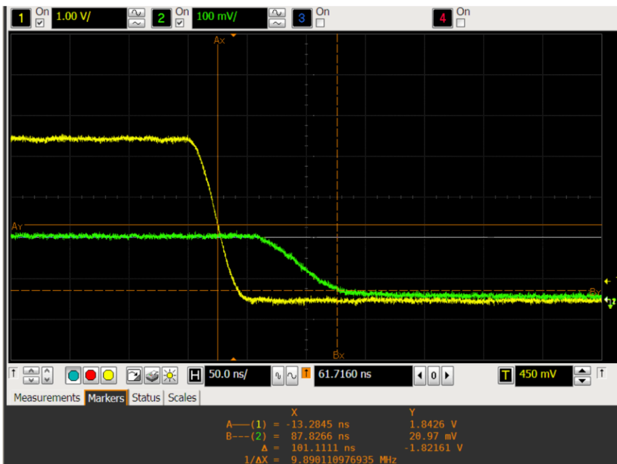
Figure 8: ERZ-HPA-0480-0490-47 RF OFF Time
