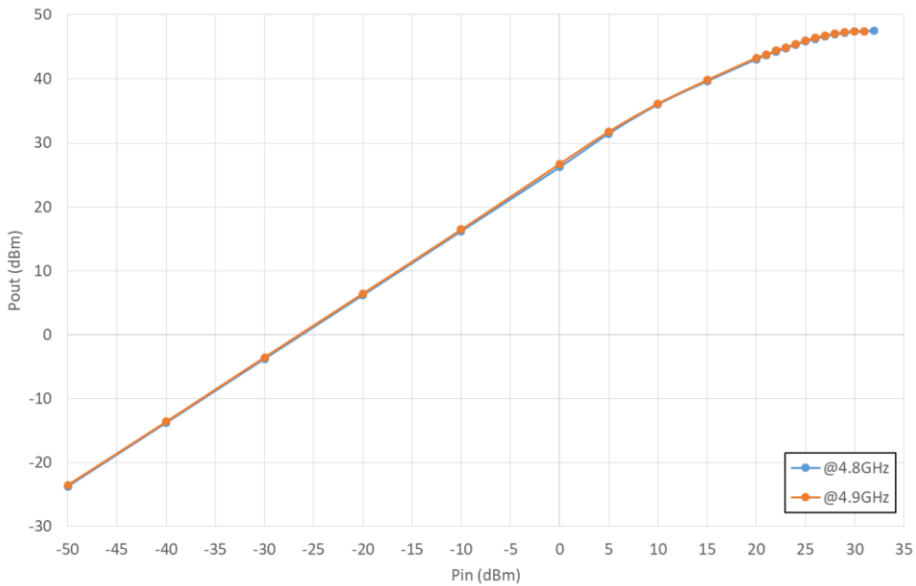
Figure 2: ERZ-HPA-0480-0490-47 Pout vs Pin
