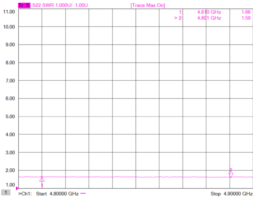
Figure 6: ERZ-HPA-0480-0490-47 Output Matching
