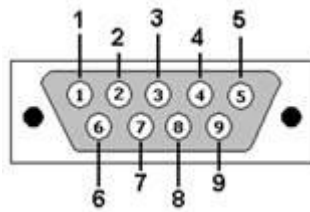
D-sub 9 Connector (Front view)
