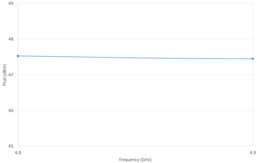
Figure 1: ERZ-HPA-0480-0490-47 Psat
