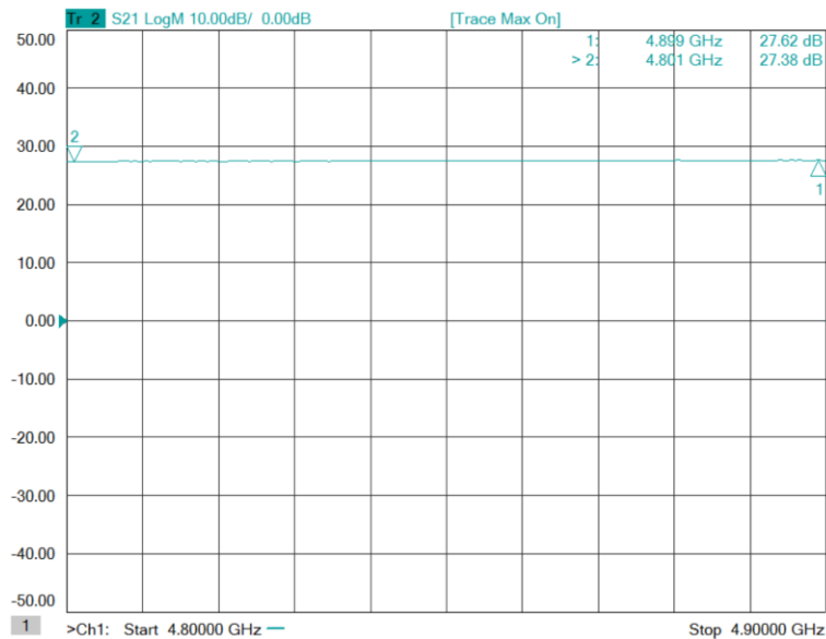
Figure 3: ERZ-HPA-0480-0490-47 Small Signal Gain
