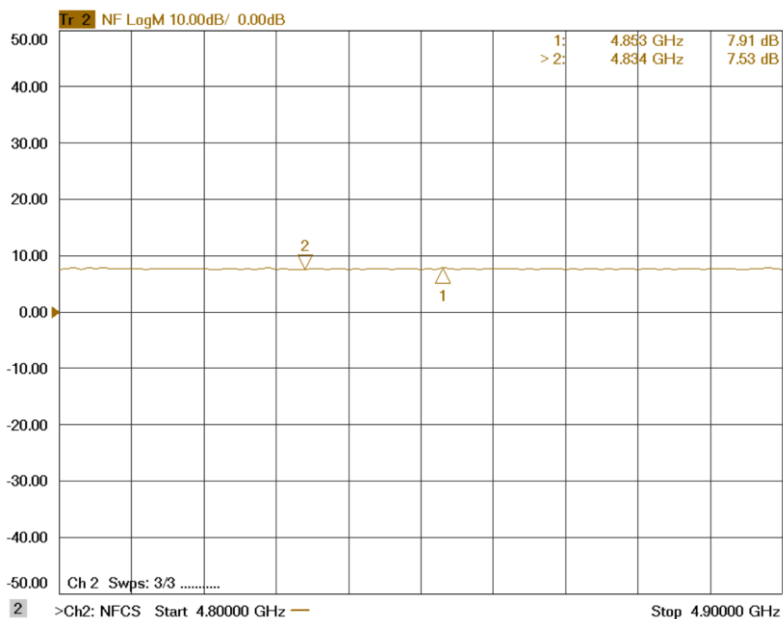
Figure 4: ERZ-HPA-0480-0490-47 Noise Figure
