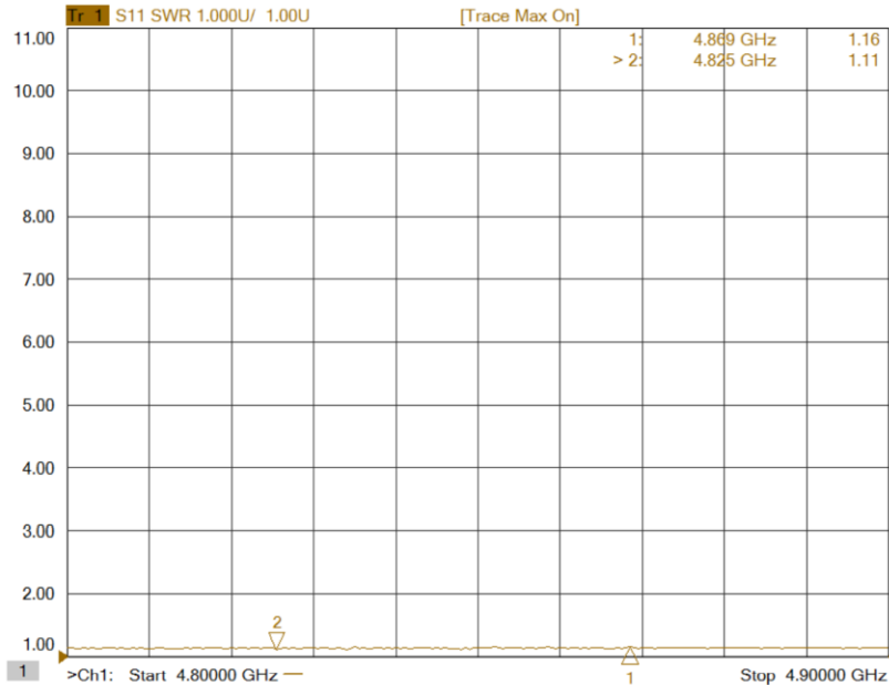
Figure 5: ERZ-HPA-0480-0490-47 Input Matching
